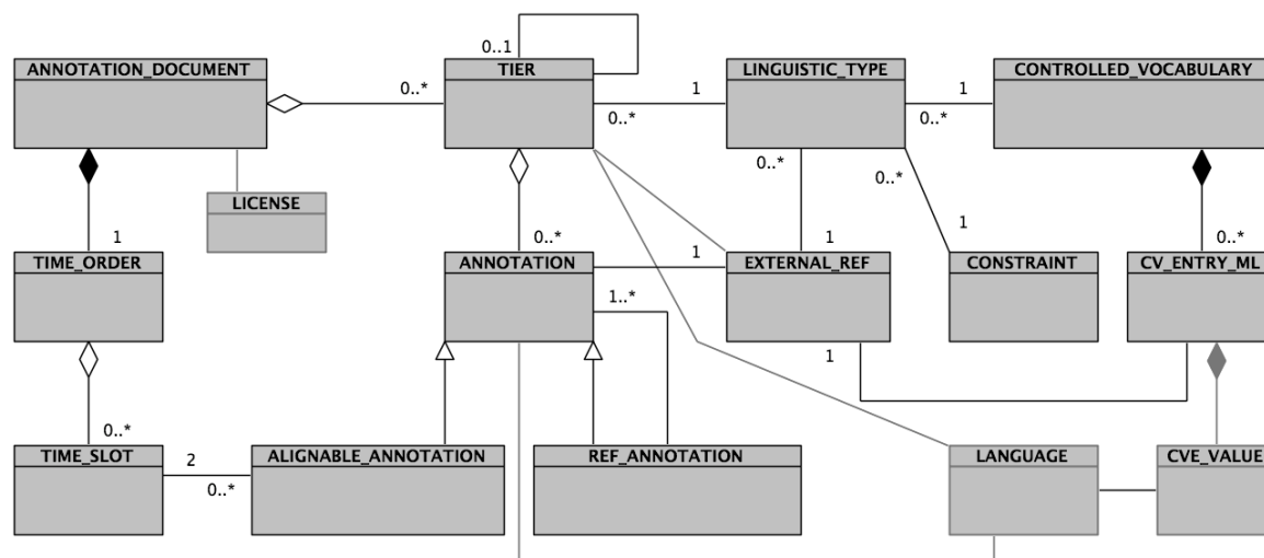
Figure 1 simplified UML class diagram
