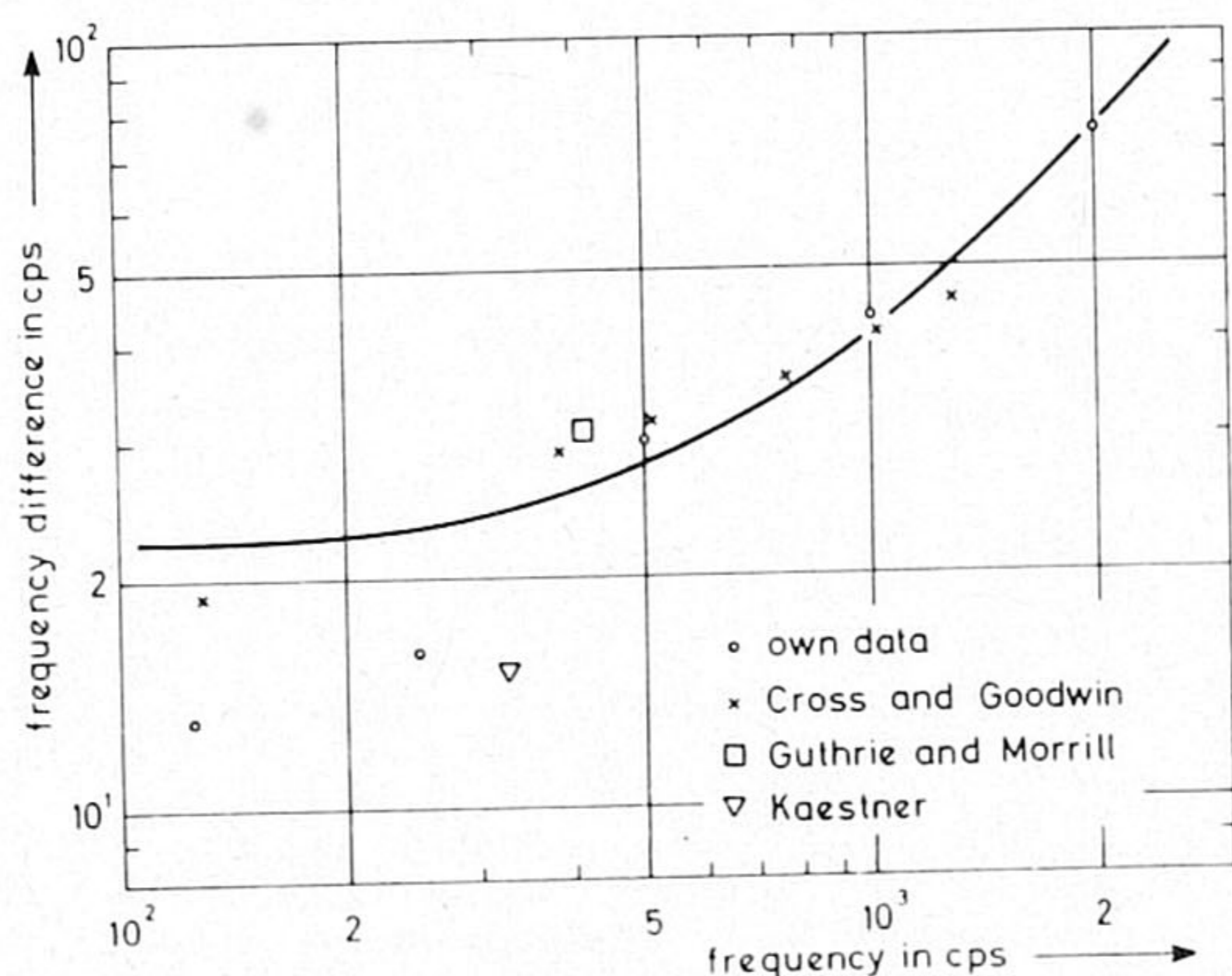
FIG. 8. Frequency difference of two simple tones for maximum dissonance as a function of the mean frequency of the tones. The solid curve corresponds with 0.25 critical bandwidth as given by Zwicker, Flottorp, and Stevens. 38
