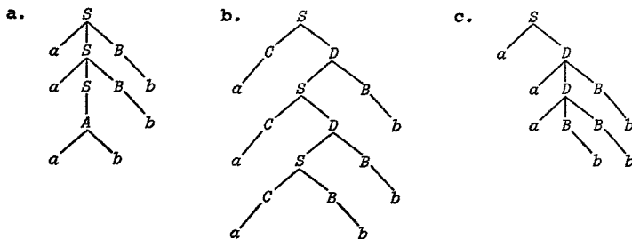
Fig. 2.3. Derivation Trees for a^3b^3 .
