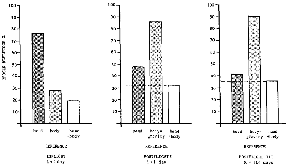
Fig. 3a and b. Percentage of chosen reference. 3a (upper) is for subject R.F.; 3b (lower) is for subject W.O. Head = verbal responses which are correct with respect to the retinal (head) coordinates. Body = verbal responses which are correct with respect to the body-defined (in zero G also the gravitational) coordinates. Head + body = verbal responses which are correct with respect to both the retinal and the body-defined coordinates, e.g. when connecting axis of the balls is 7° and the head is tilted to the right by approximately 30 to 35°, the correct description with respect to each of the coordinates would be "right above."
